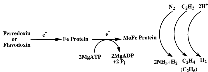
Fig. 1. Electron transfer path for molybdenum nitrogenase.
